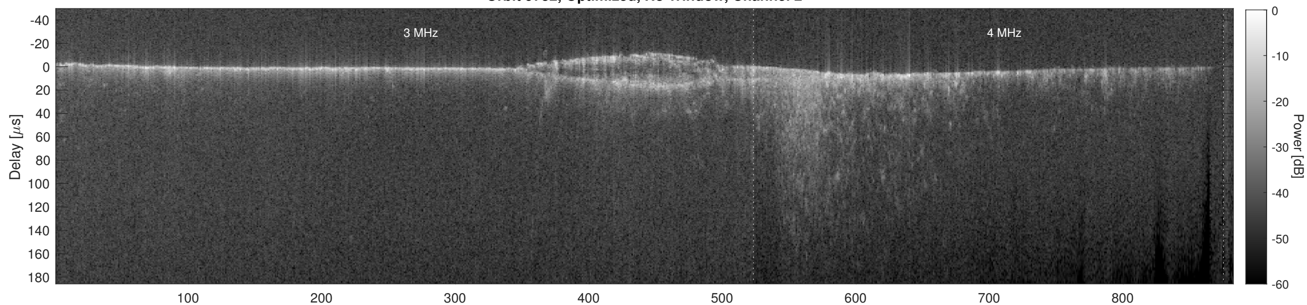
Orbit 9732, Cluttergram
