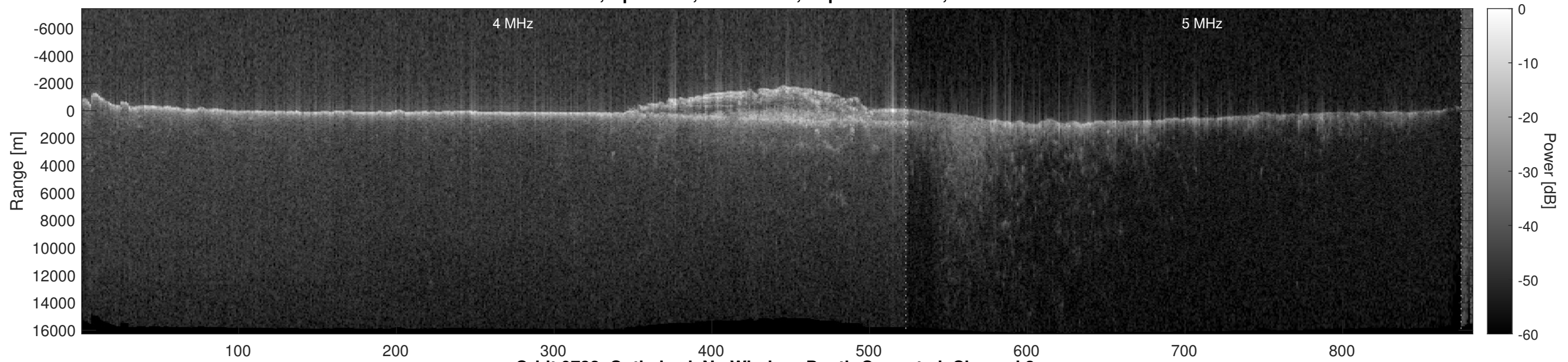
Orbit 9732, Optimized, No Window, Depth-Corrected, Channel 2
