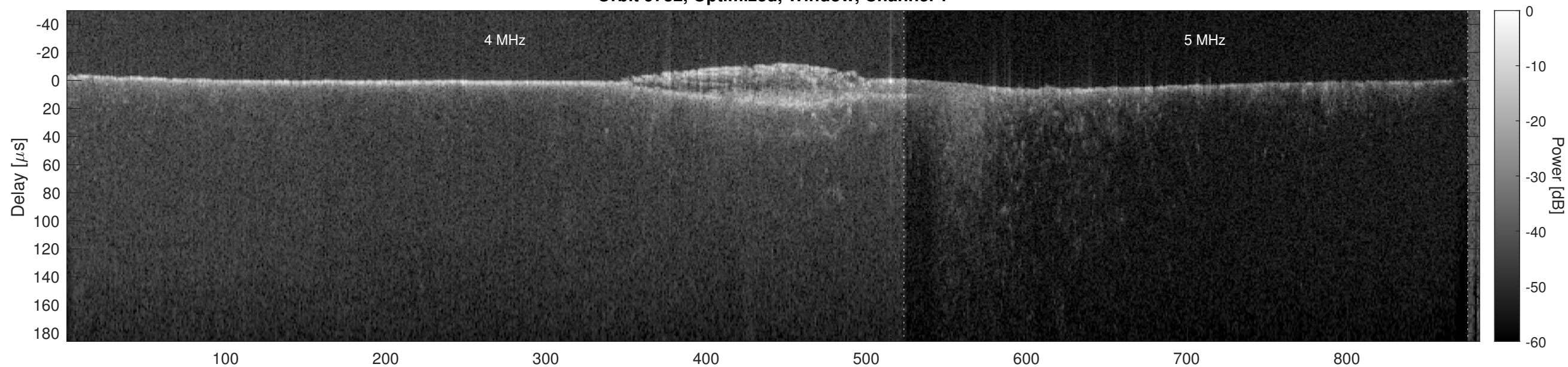
Orbit 9732, Optimized, Window, Channel 2
