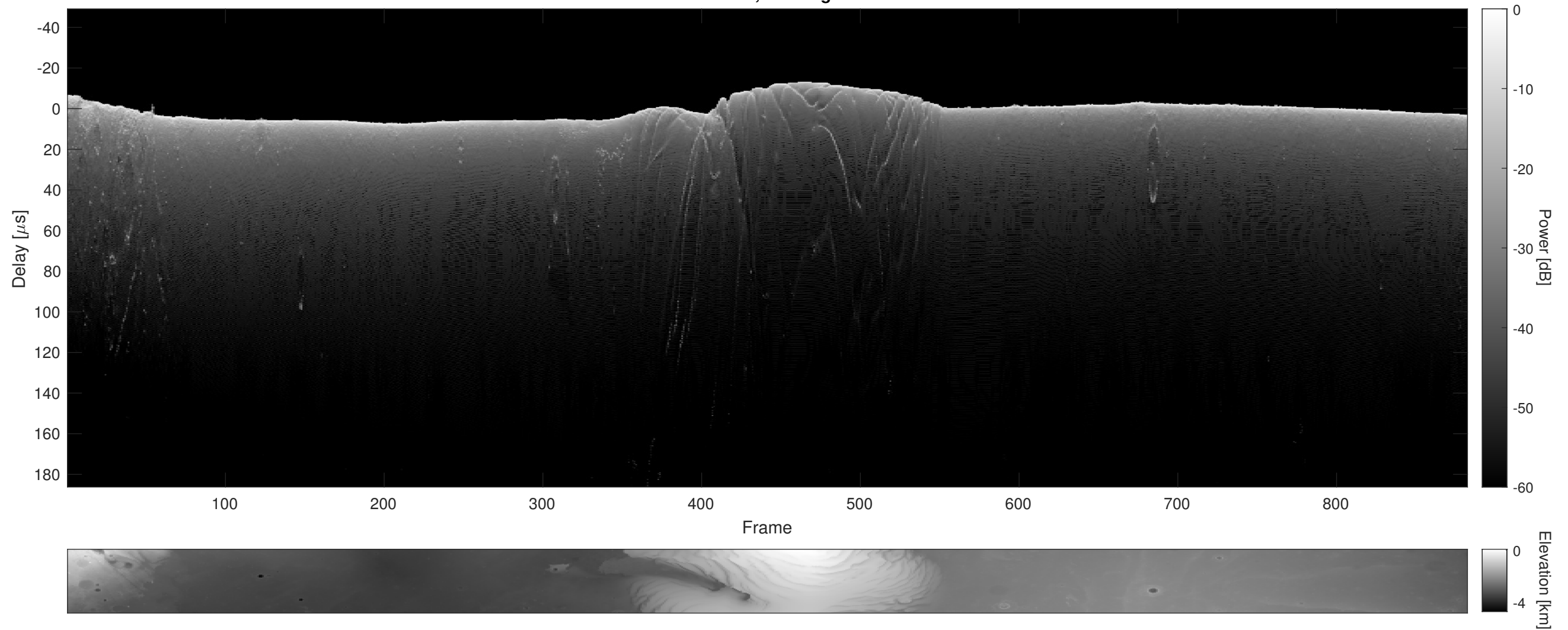
Orbit 9733, Cluttergram
