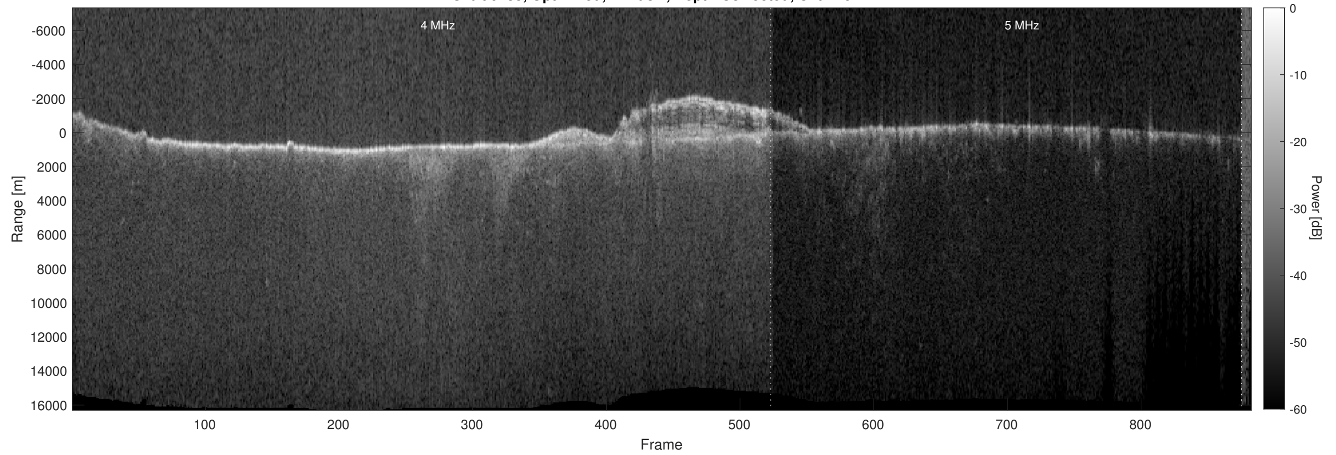
Orbit 9733, Optimized, Window, Depth-Corrected, Channel 2
