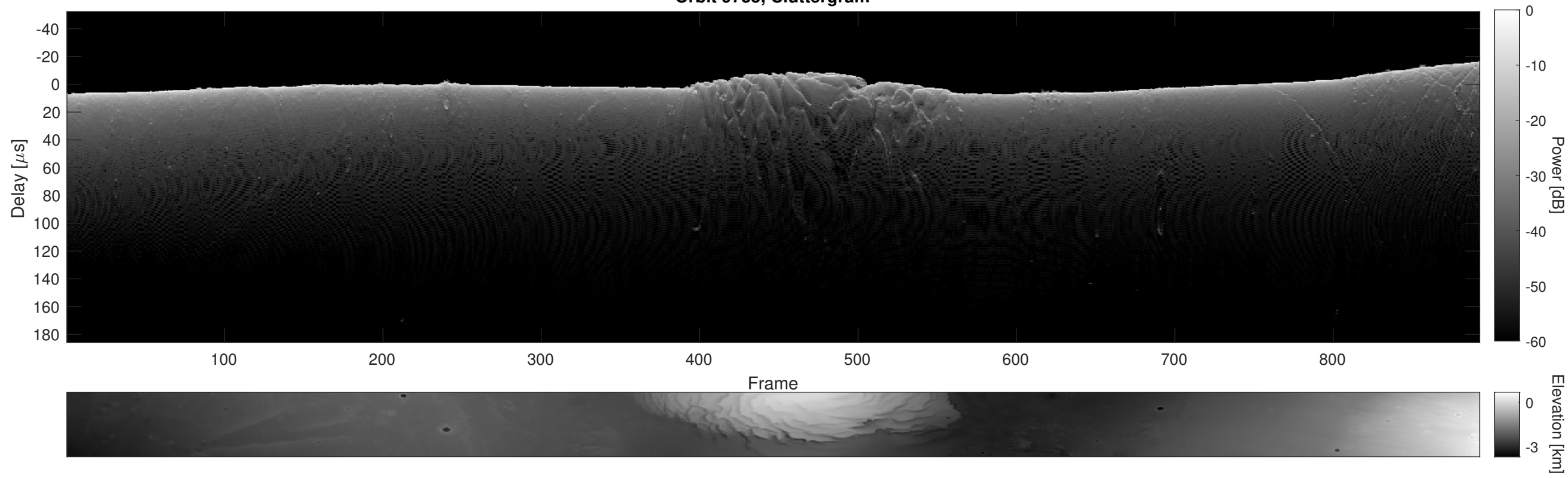
Orbit 9735, Cluttergram
