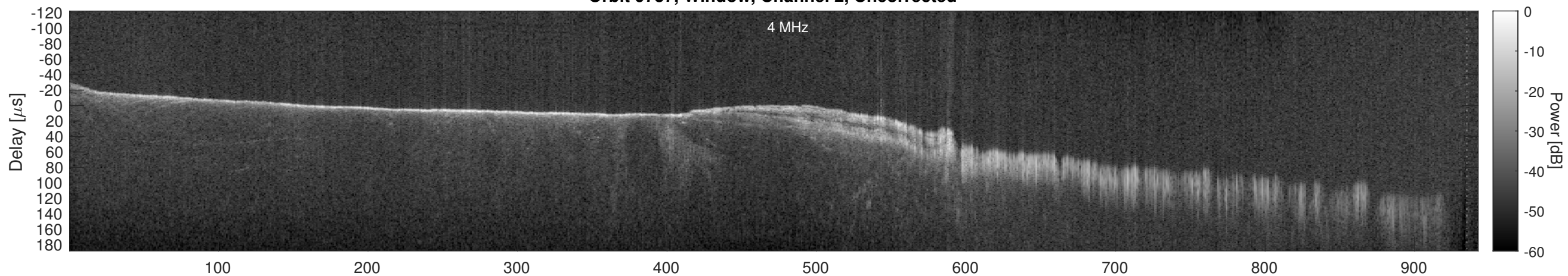
Orbit 9737, Window, Channel 2, Chapman
