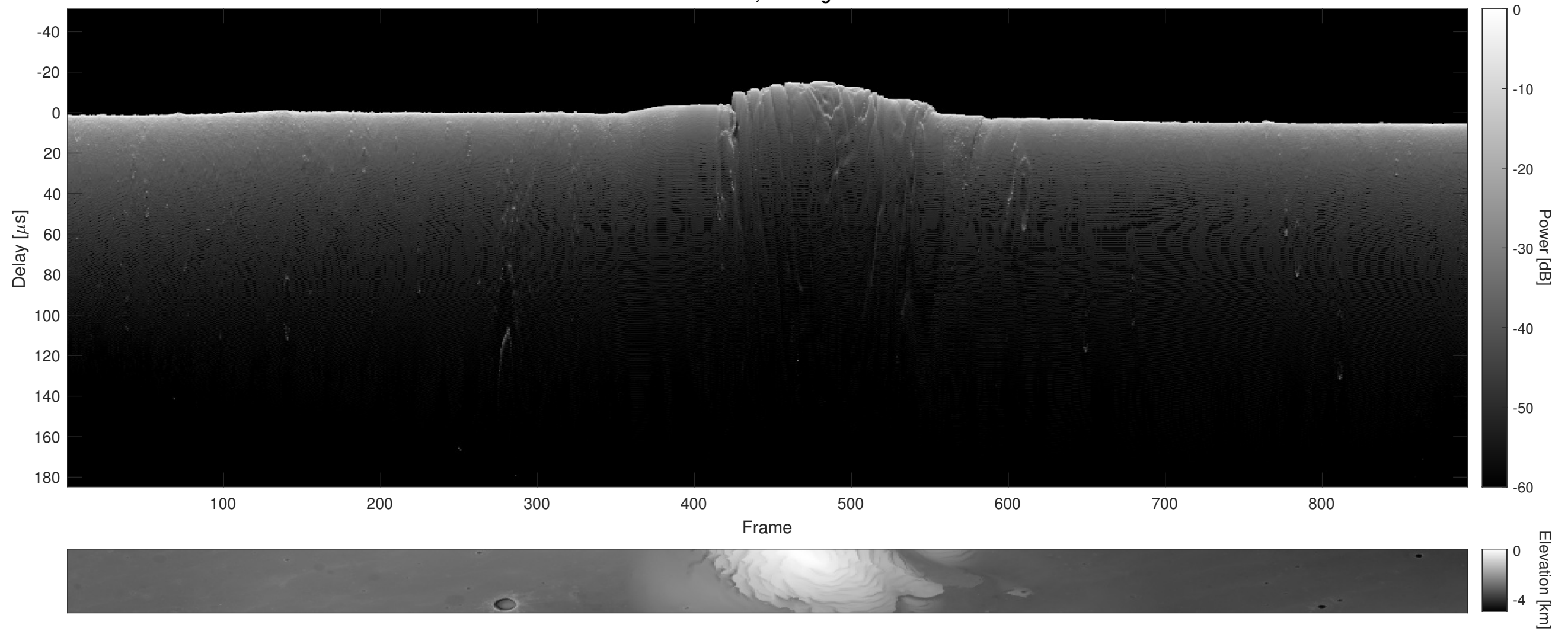
Orbit 9738, Cluttergram
