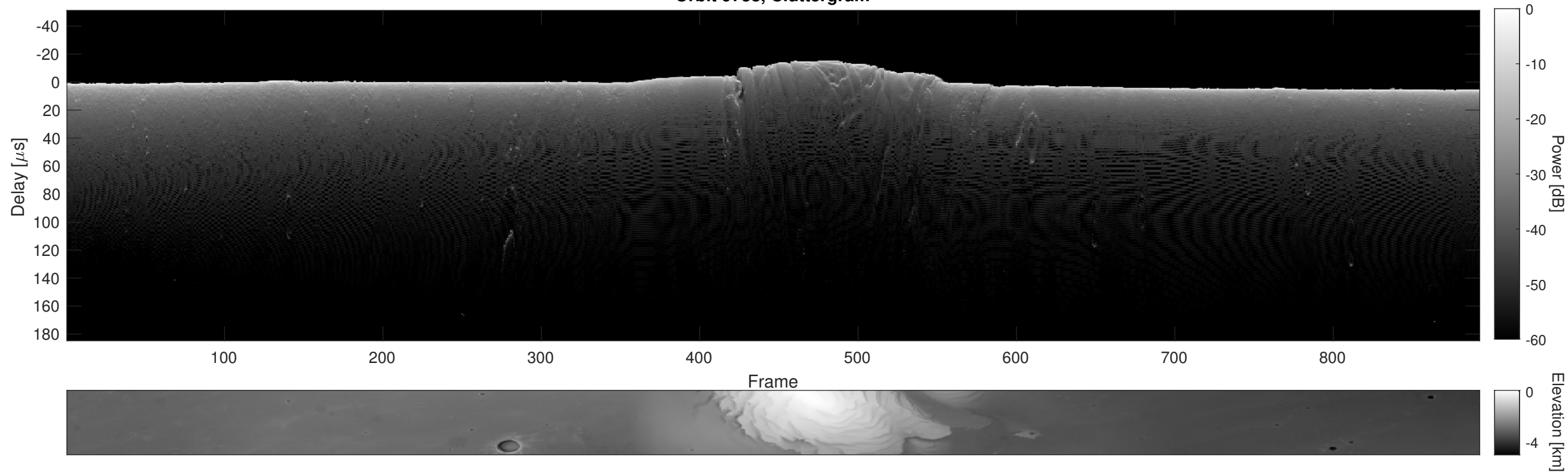
Orbit 9738, Cluttergram
