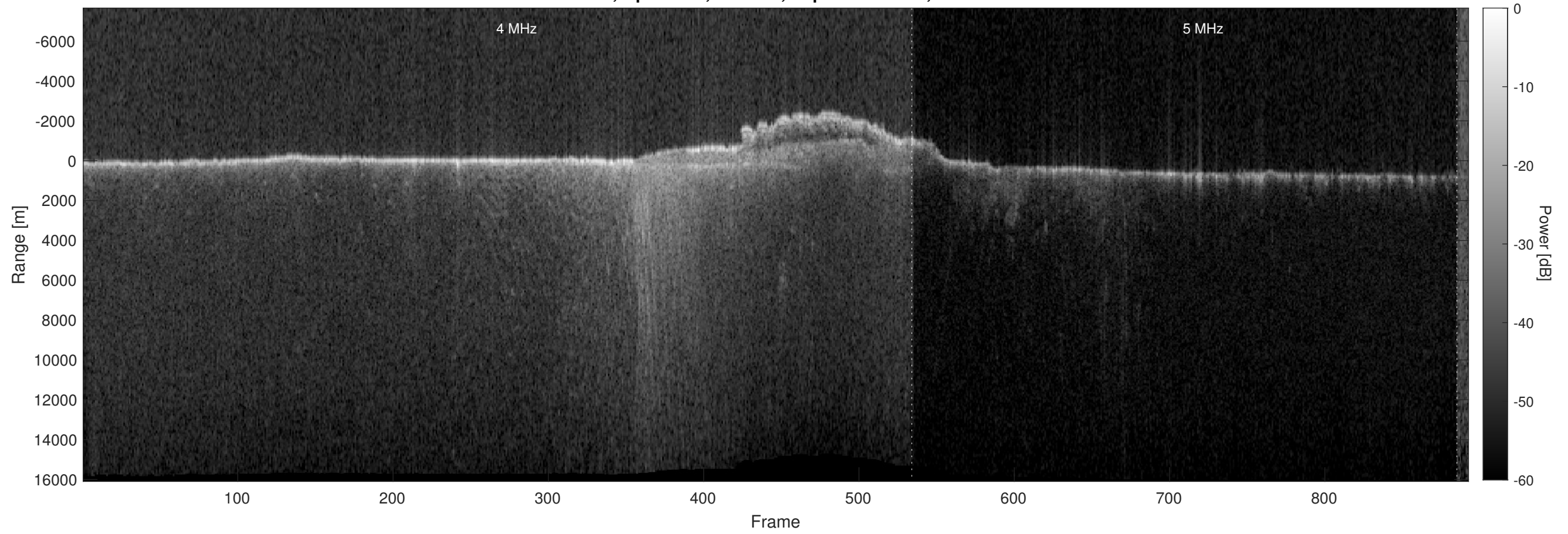
Orbit 9738, Optimized, Window, Depth-Corrected, Channel 2
