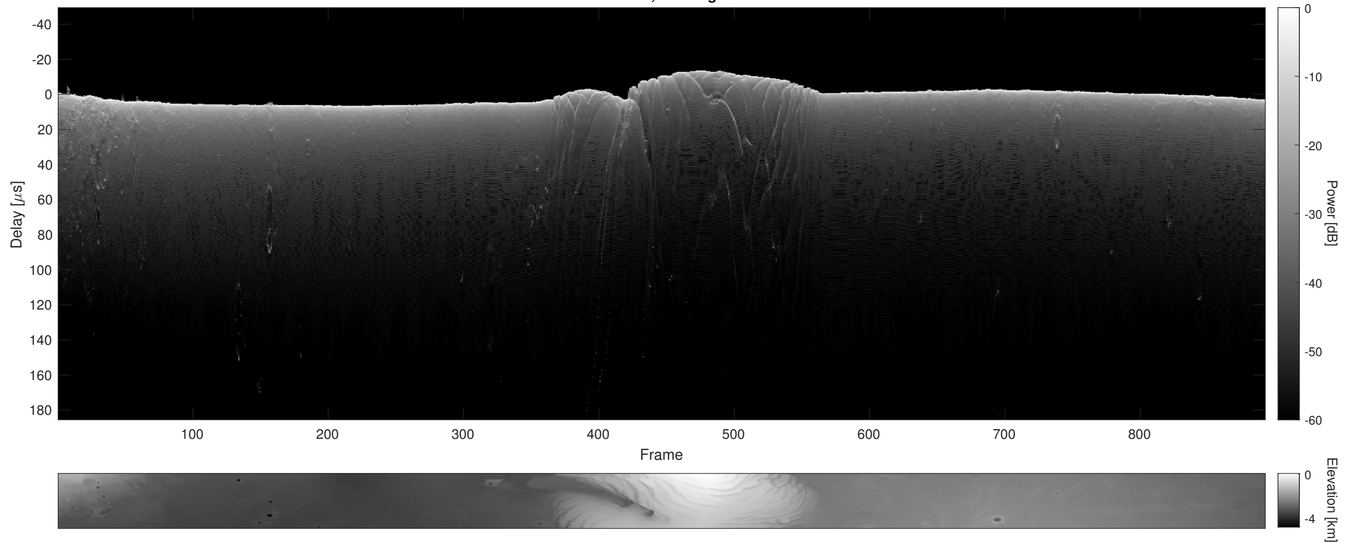
Orbit 9740, Cluttergram
