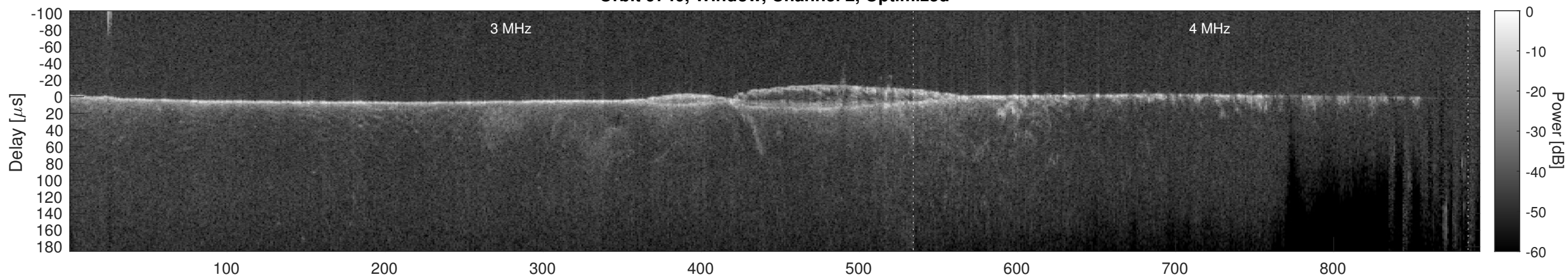
Orbit 9740, Cluttergram
