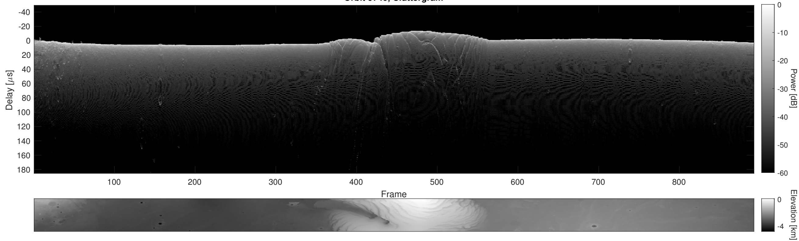
Orbit 9740, Cluttergram
