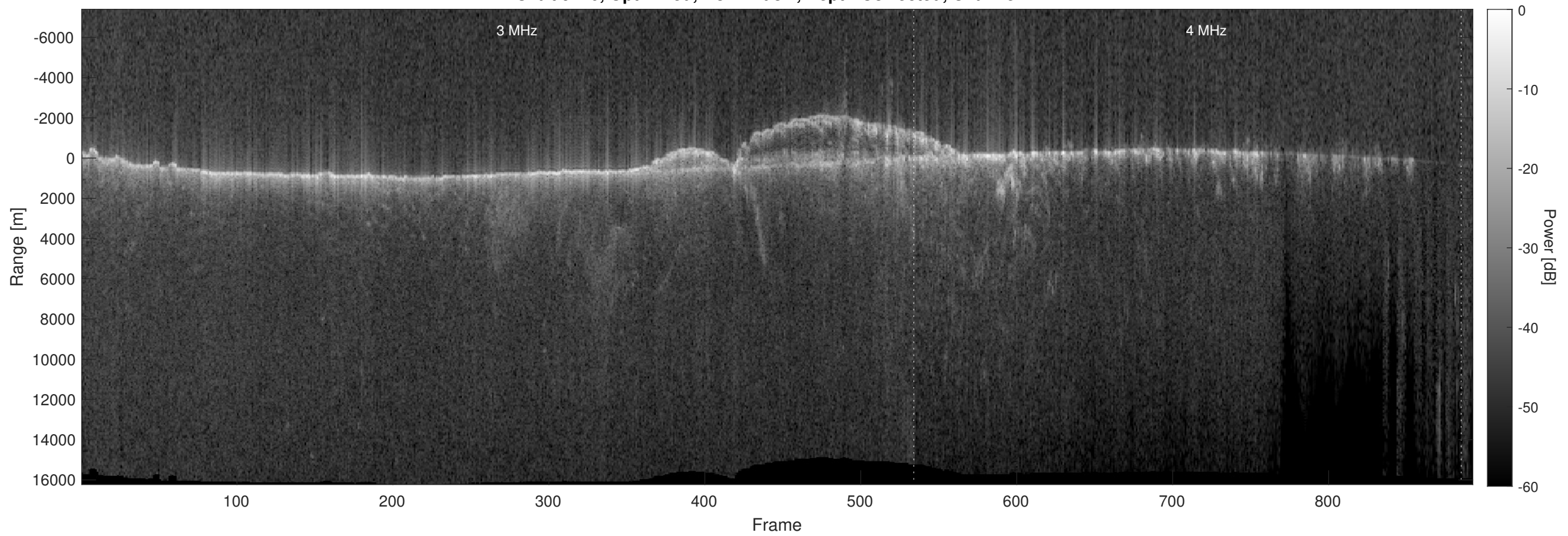
Orbit 9740, Optimized, No Window, Depth-Corrected, Channel 2
