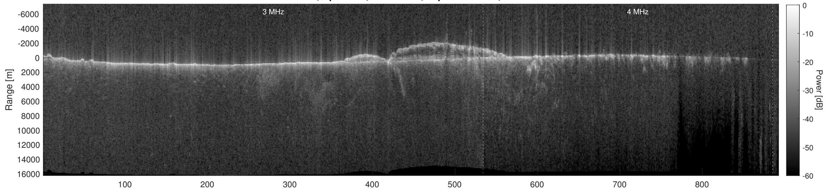
Orbit 9740, Depth-Corrected Cluttergram
