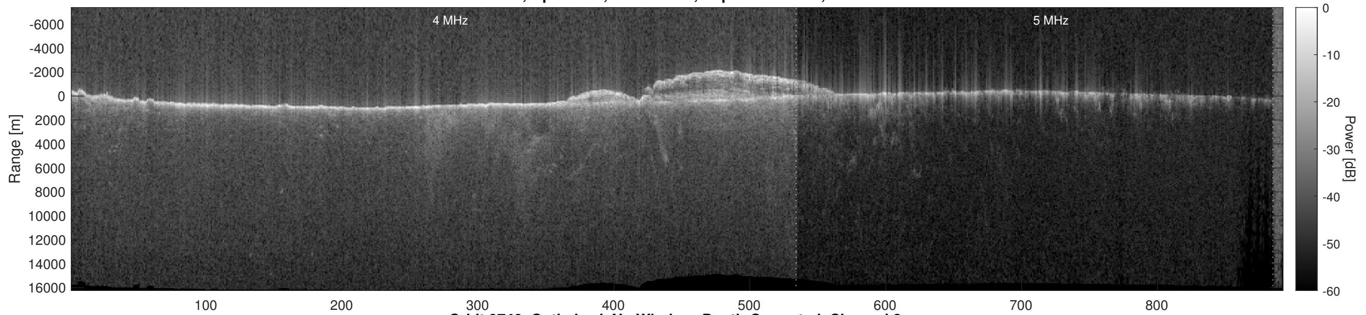
Orbit 9740, Optimized, No Window, Depth-Corrected, Channel 2
