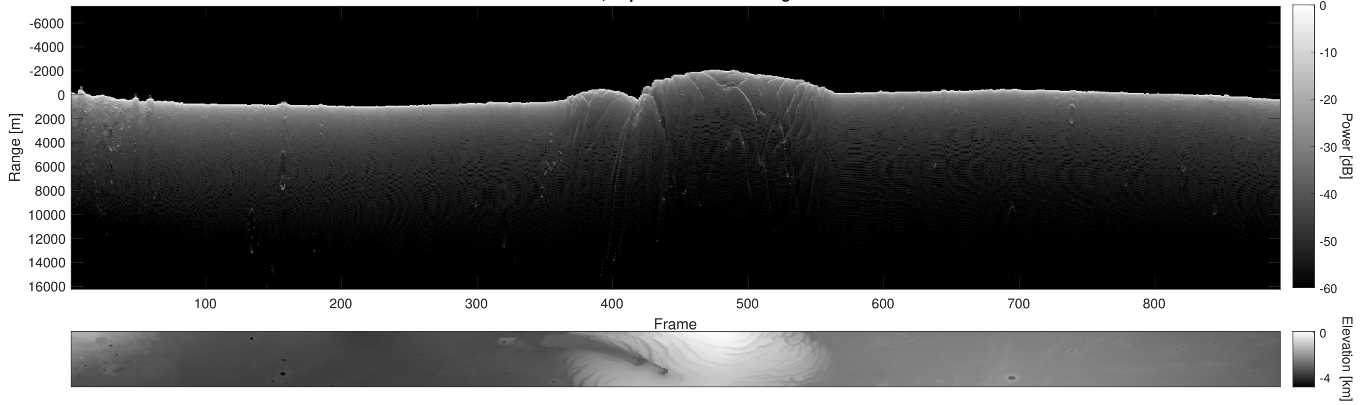
Orbit 9740, Depth-Corrected Cluttergram
