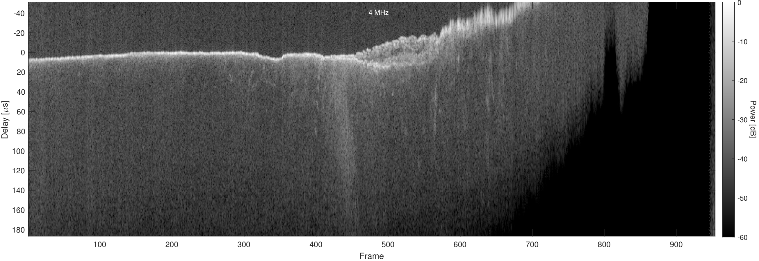
Orbit 9742, Chapman, Window, Channel 2
