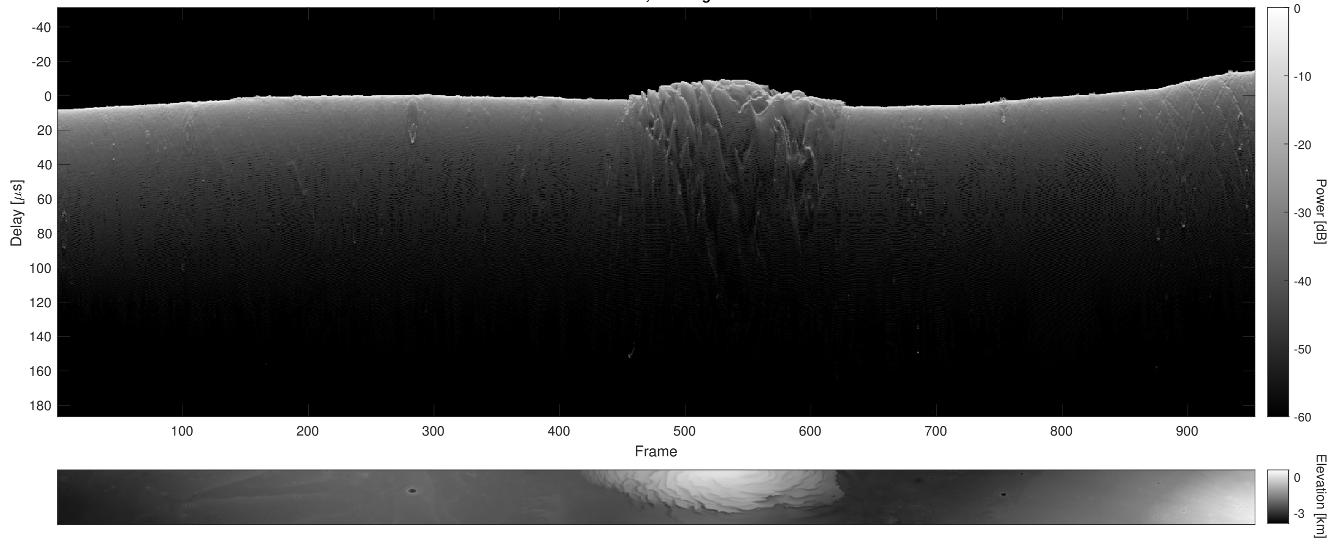
Orbit 9742, Cluttergram
