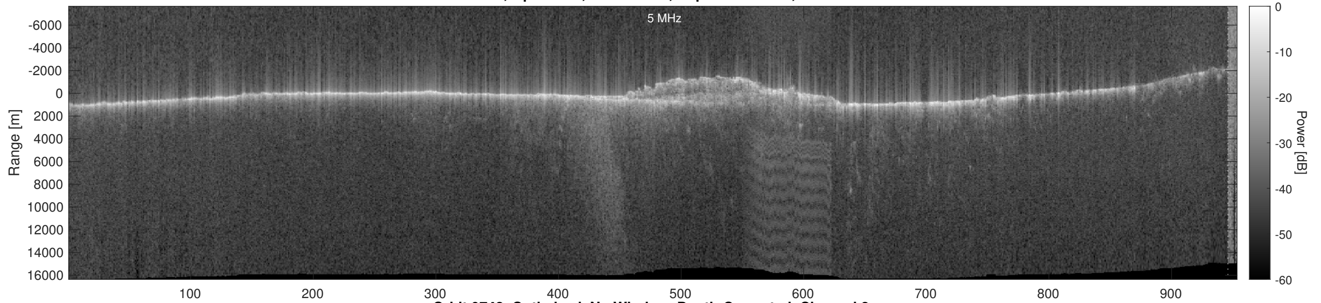
Orbit 9742, Optimized, No Window, Depth-Corrected, Channel 2
