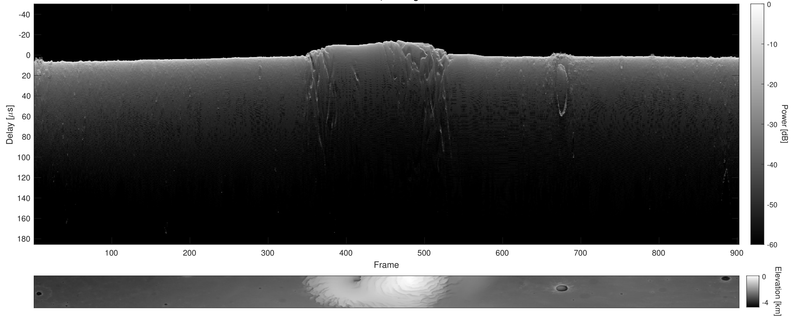
Orbit 9743, Cluttergram
