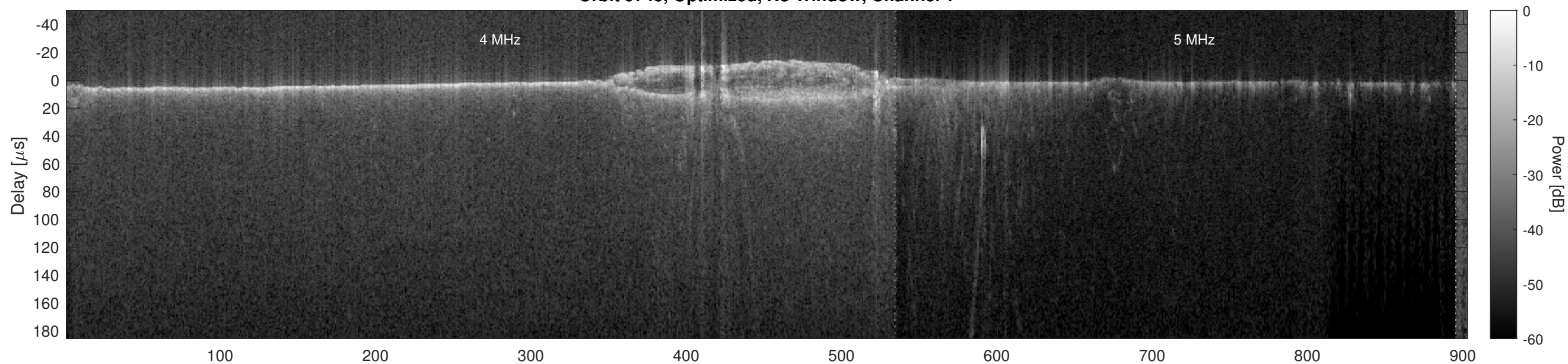
Orbit 9743, Optimized, No Window, Channel 2
