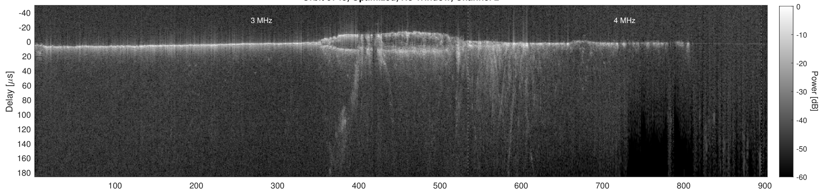
Orbit 9743, Cluttergram
