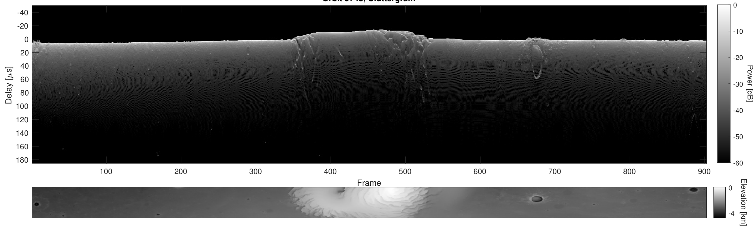
Orbit 9743, Cluttergram
