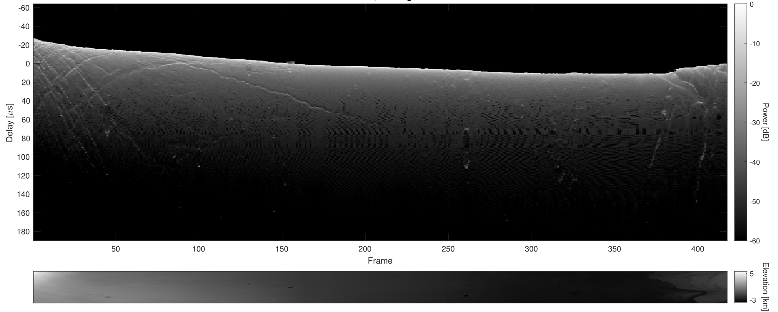
Orbit 9744, Cluttergram
