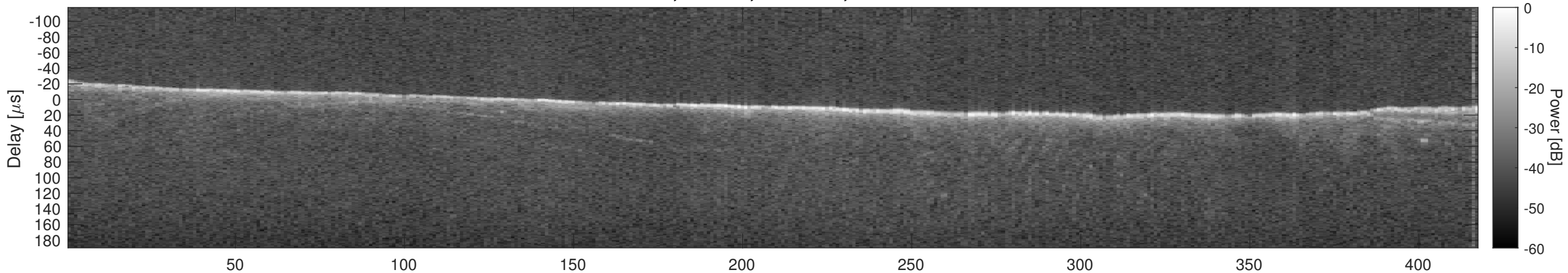
Orbit 9744, Window, Channel 2, Chapman
