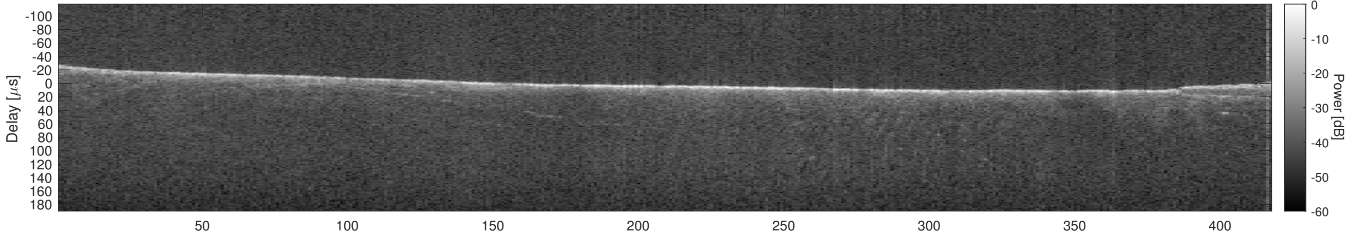
Orbit 9744, Cluttergram
