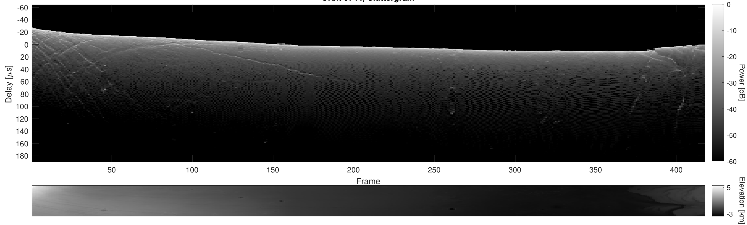
Orbit 9744, Cluttergram
