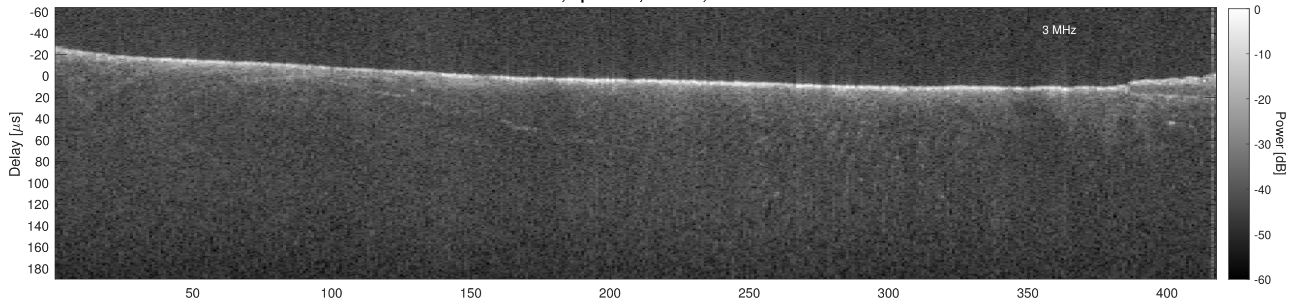
Orbit 9744, Cluttergram
