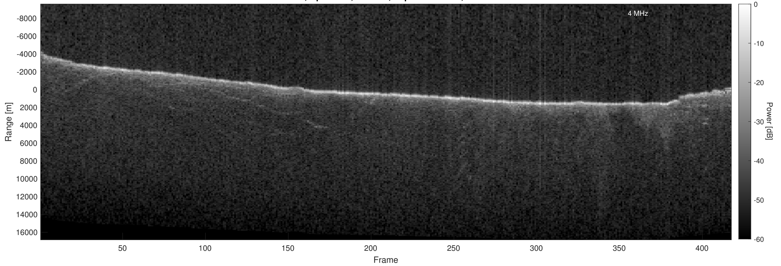
Orbit 9744, Optimized, Window, Depth-Corrected, Channel 2
