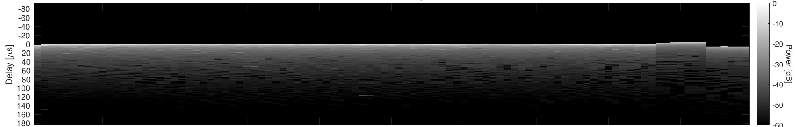
Orbit 9745, Cluttergram
