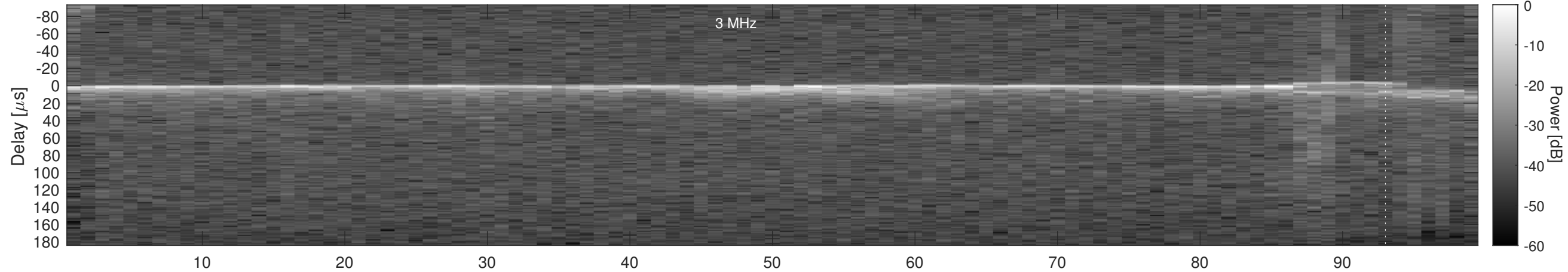
Orbit 9745, Cluttergram
