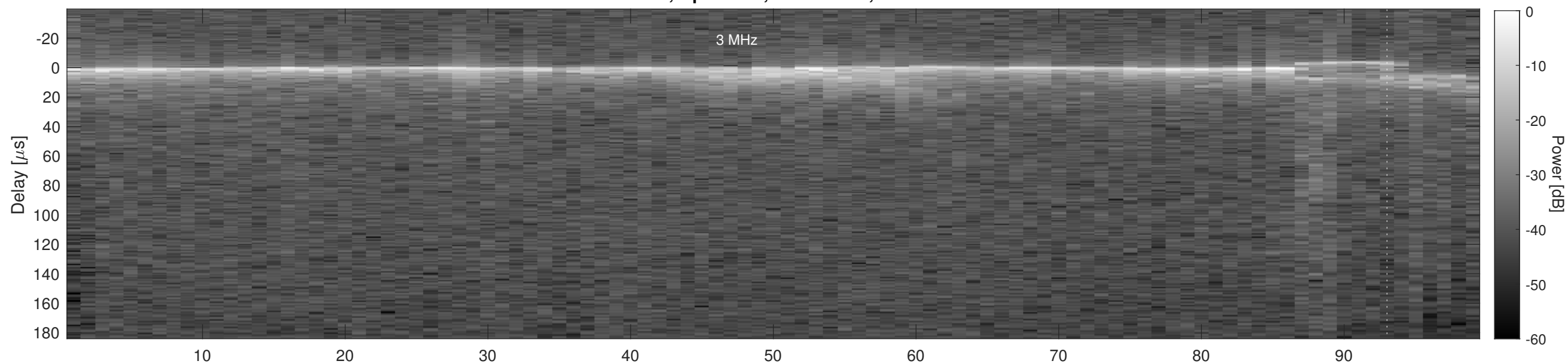
Orbit 9745, Cluttergram
