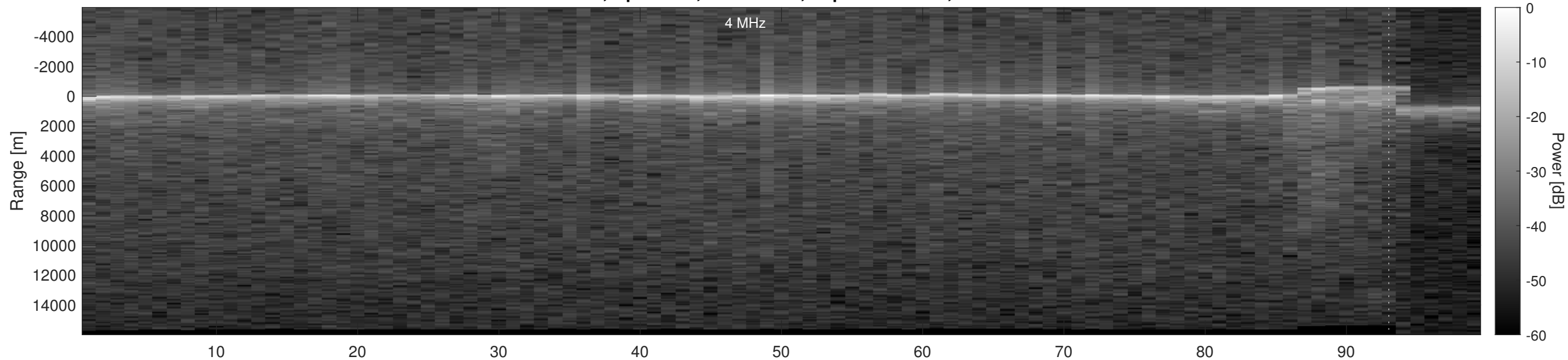
Orbit 9745, Optimized, No Window, Depth-Corrected, Channel 2
