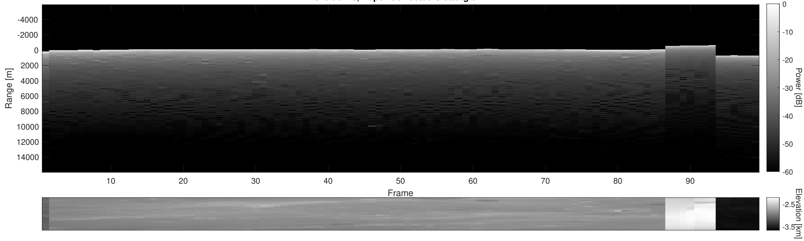
Orbit 9745, Depth-Corrected Cluttergram
