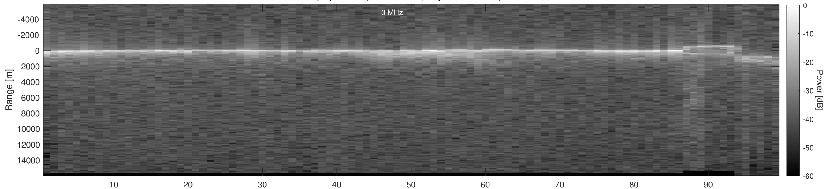
Orbit 9745, Depth-Corrected Cluttergram
