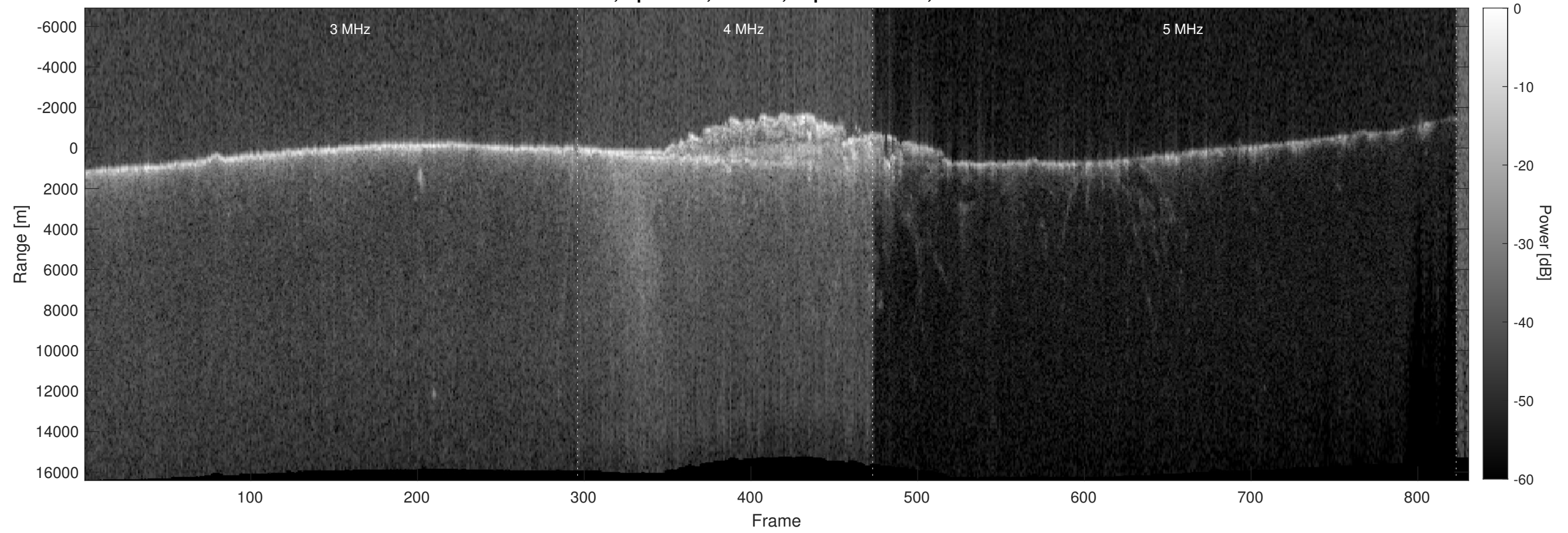
Orbit 9749, Optimized, Window, Depth-Corrected, Channel 2
