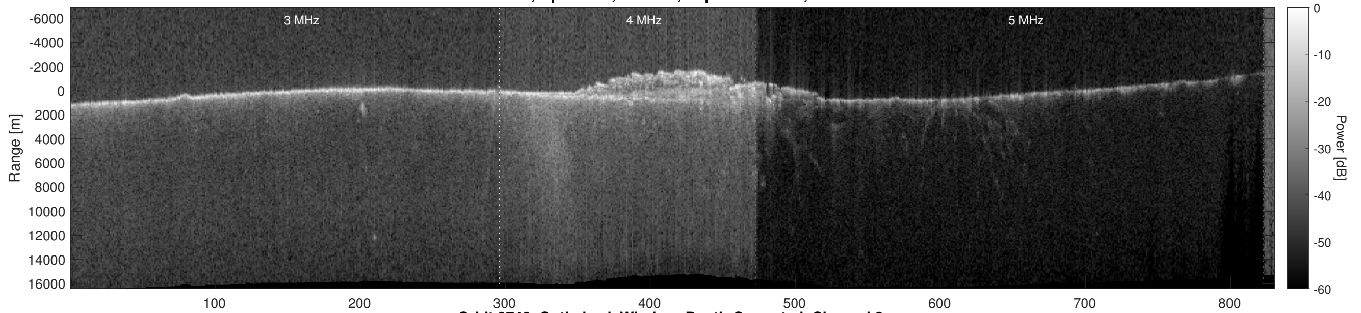
Orbit 9749, Optimized, Window, Depth-Corrected, Channel 2
