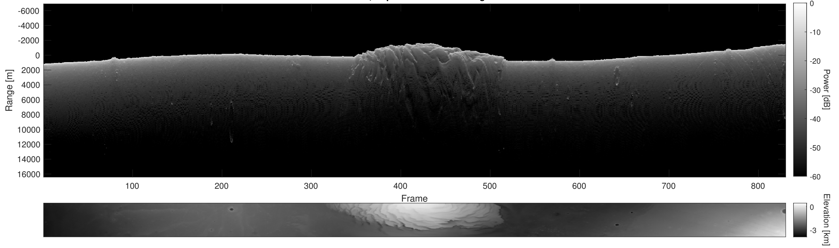
Orbit 9749, Depth-Corrected Cluttergram
