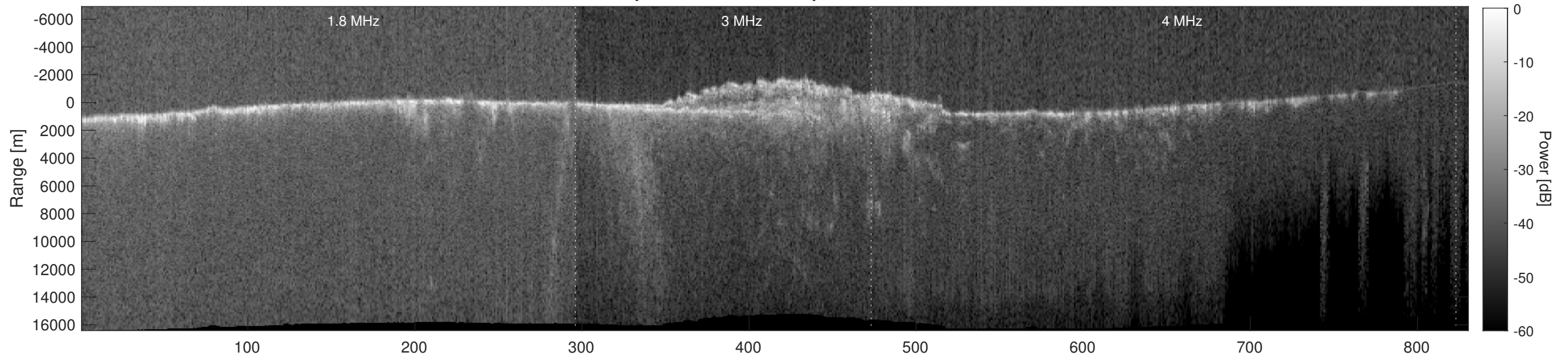
Orbit 9749, Depth-Corrected Cluttergram
