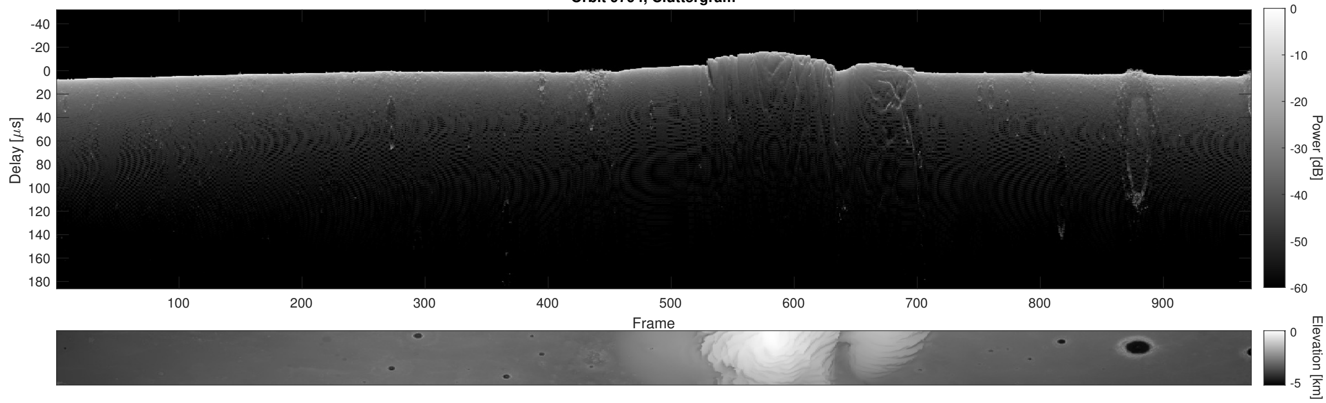
Orbit 9794, Cluttergram
