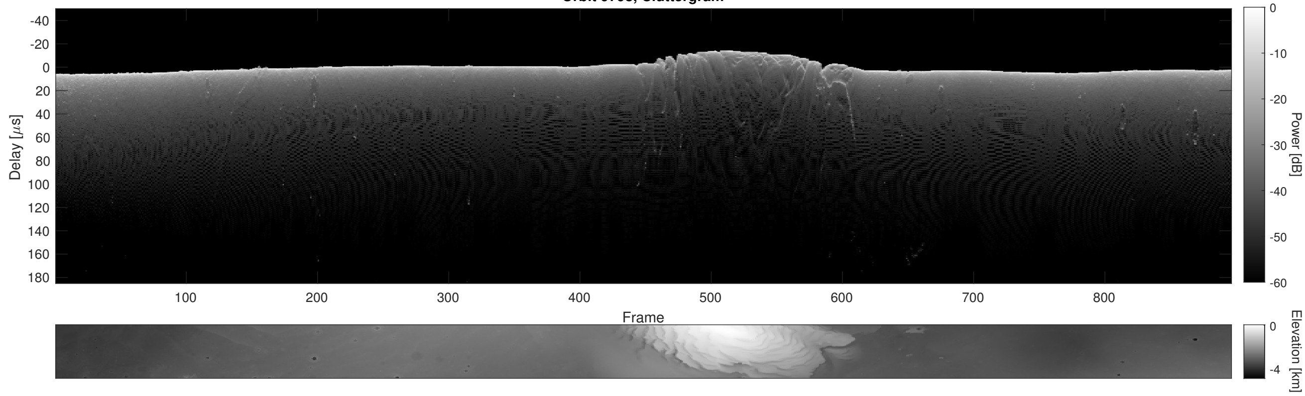
Orbit 9798, Cluttergram
