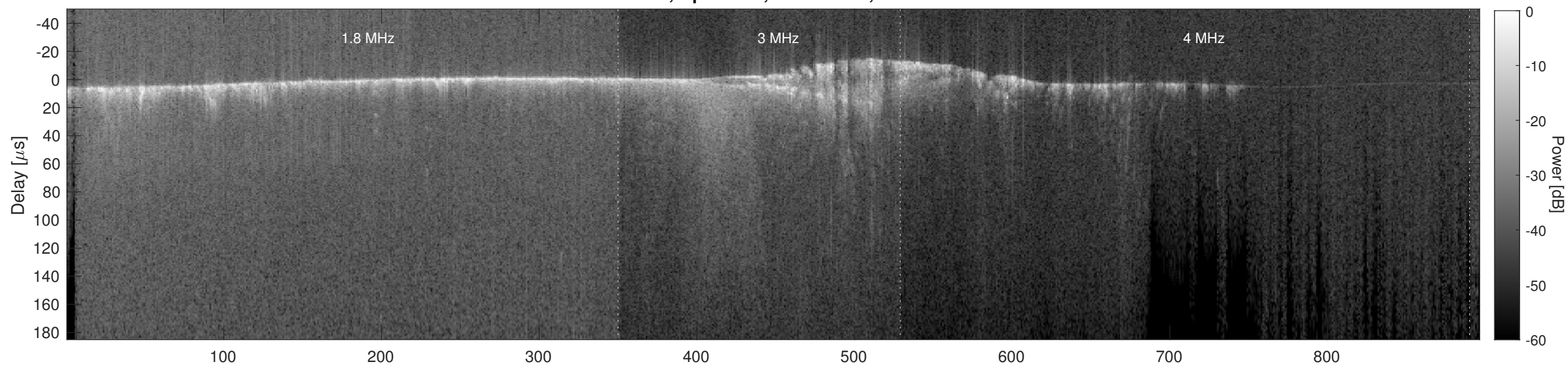
Orbit 9798, Cluttergram
