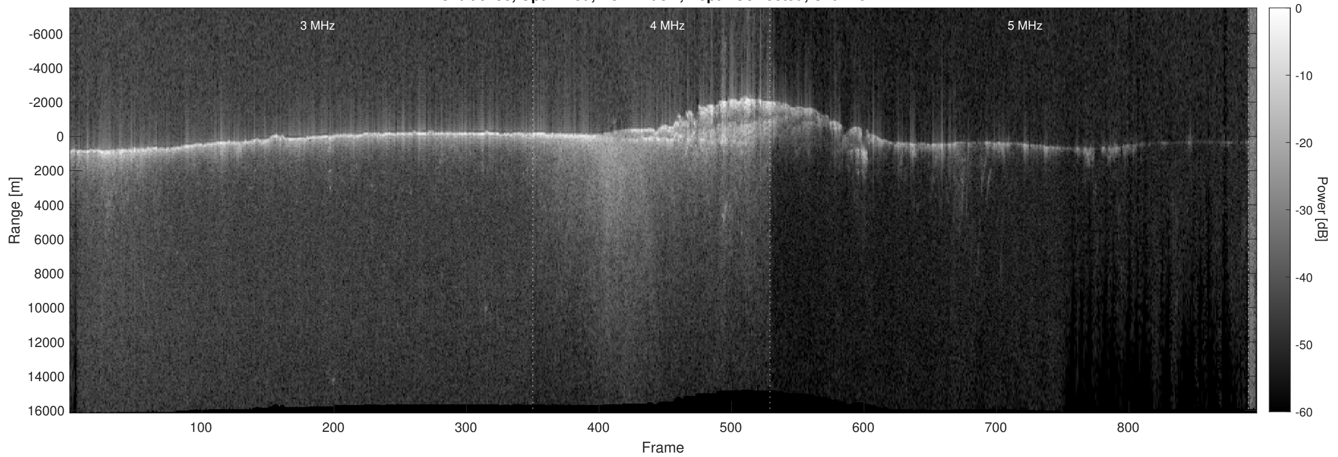
Orbit 9798, Optimized, No Window, Depth-Corrected, Channel 2
