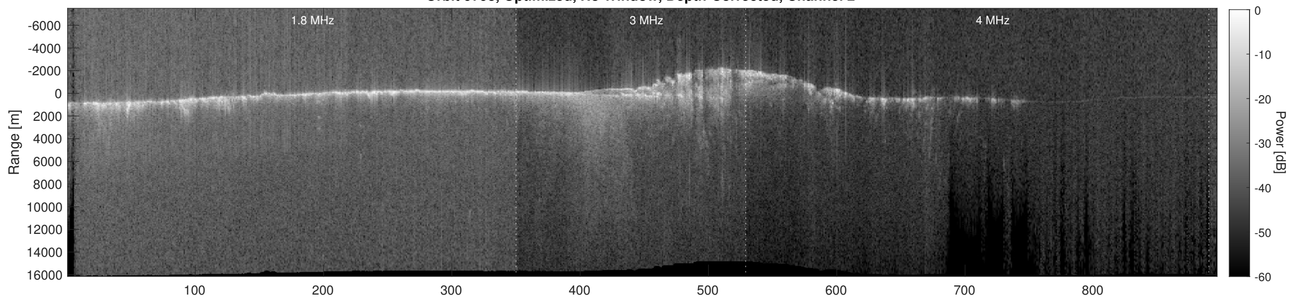
Orbit 9798, Depth-Corrected Cluttergram
