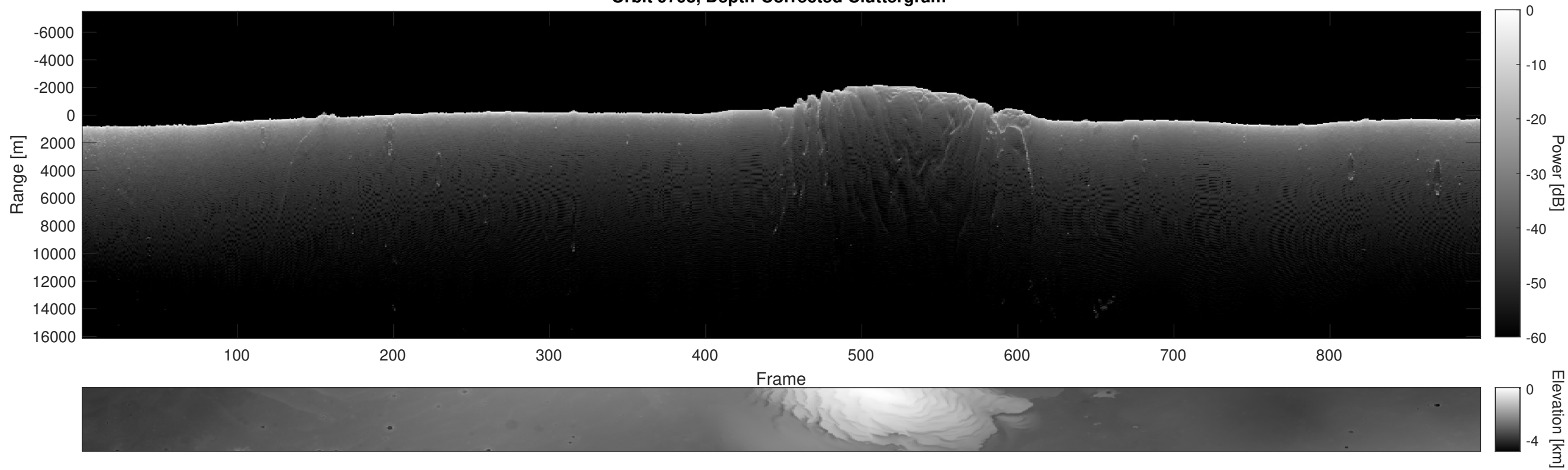
Orbit 9798, Depth-Corrected Cluttergram
