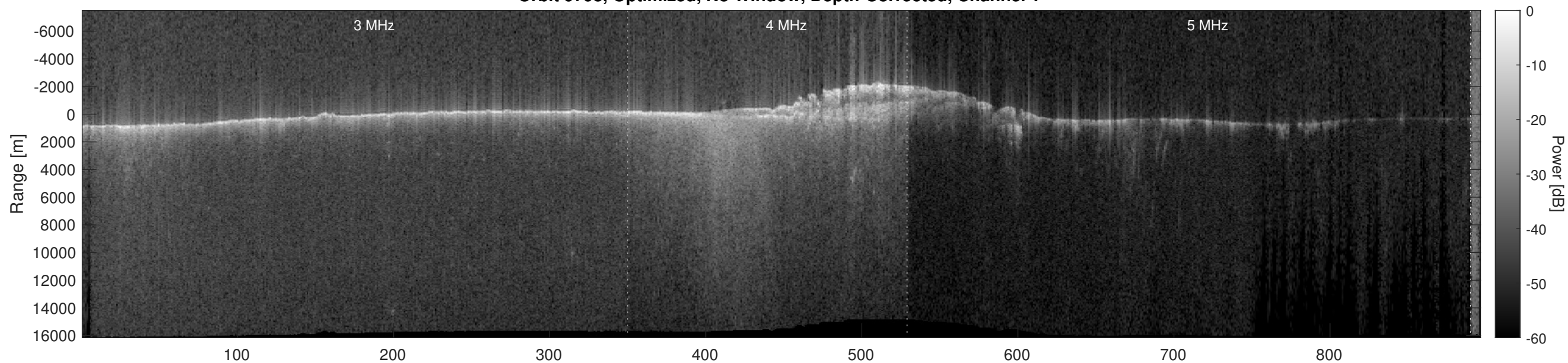
Orbit 9798, Optimized, No Window, Depth-Corrected, Channel 2
