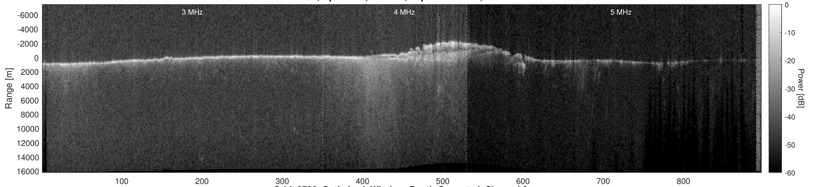
Orbit 9798, Optimized, Window, Depth-Corrected, Channel 2
