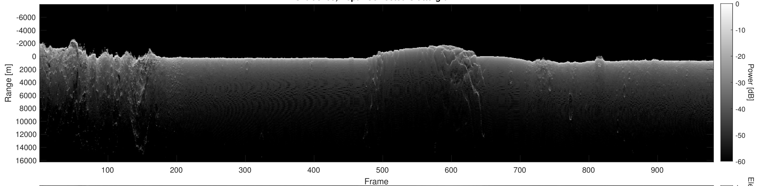
Orbit 9799, Depth-Corrected Cluttergram
