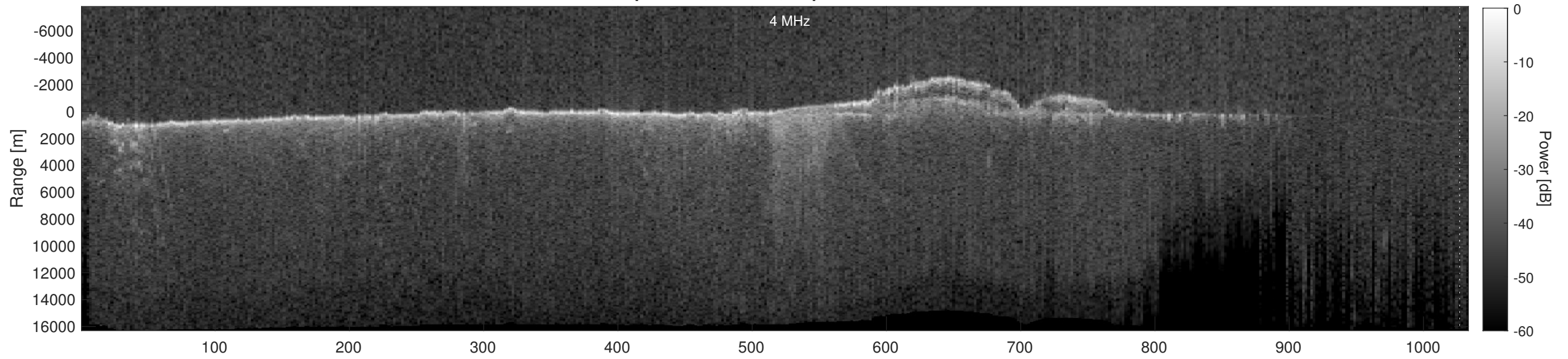
Orbit 9801, Depth-Corrected Cluttergram
