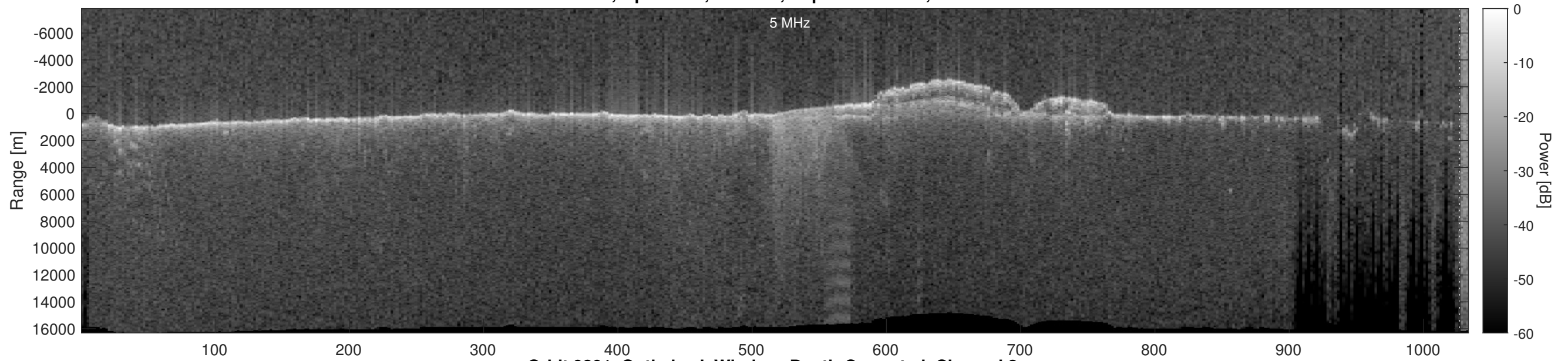
Orbit 9801, Optimized, Window, Depth-Corrected, Channel 2
