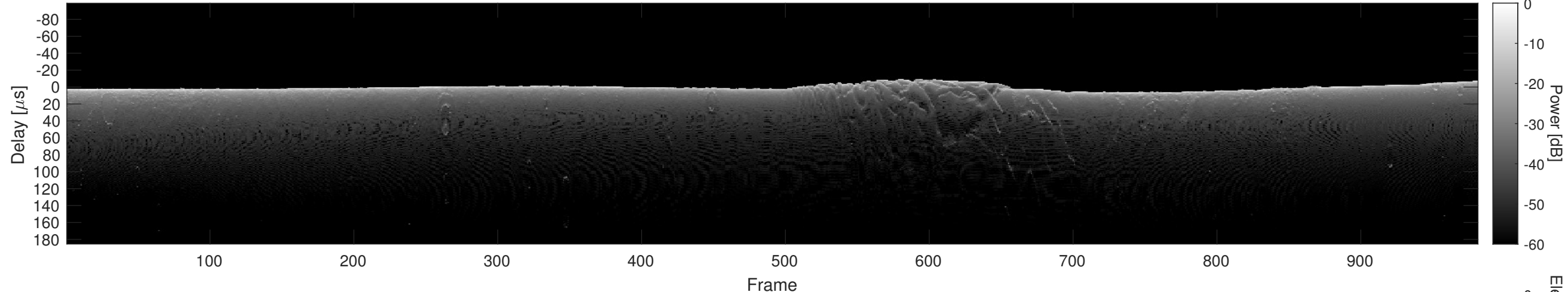
Orbit 9802, Cluttergram
