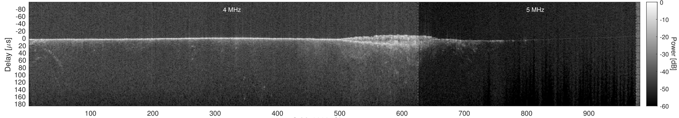
Orbit 9802, Cluttergram
