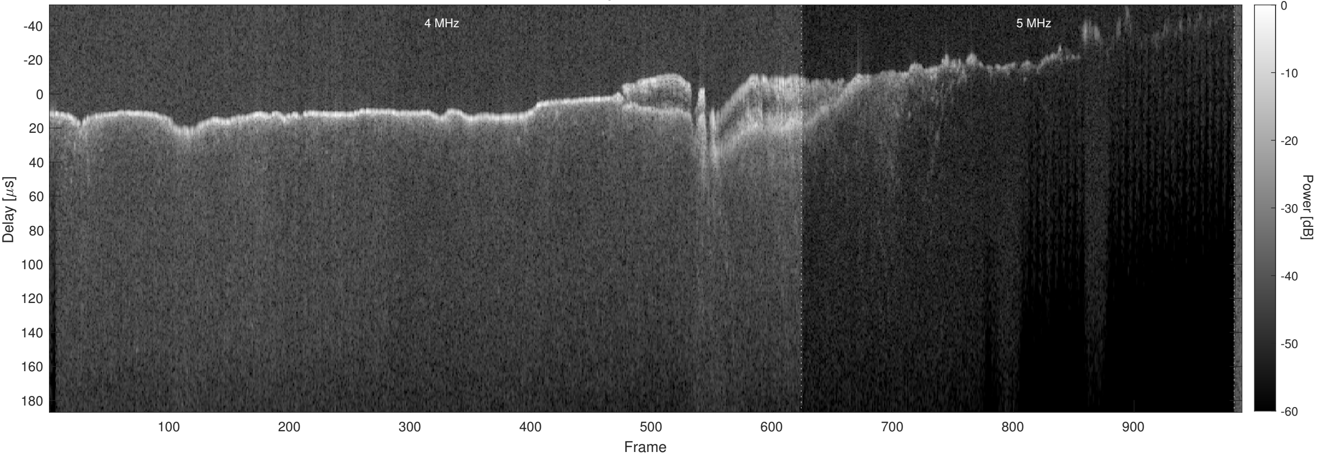
Orbit 9803, Chapman, Window, Channel 2
