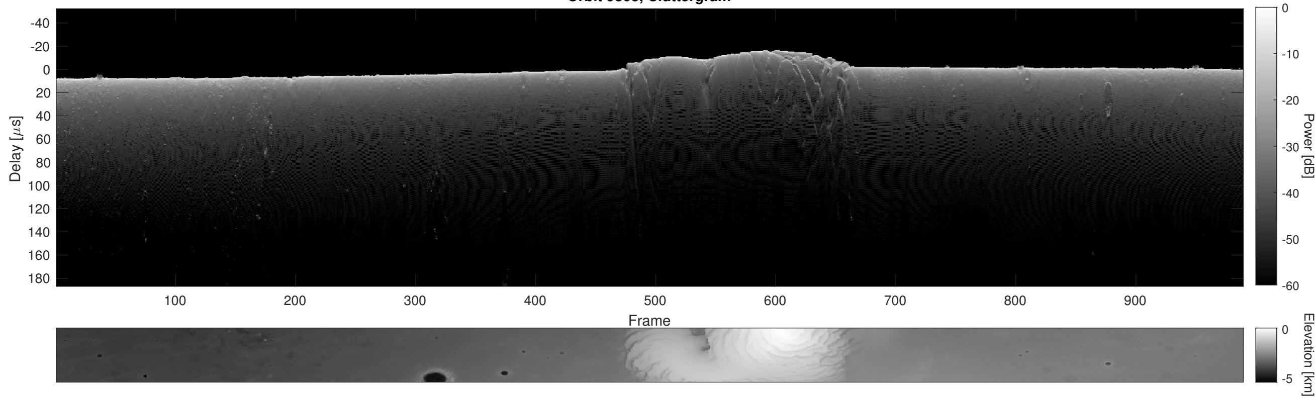
Orbit 9803, Cluttergram
