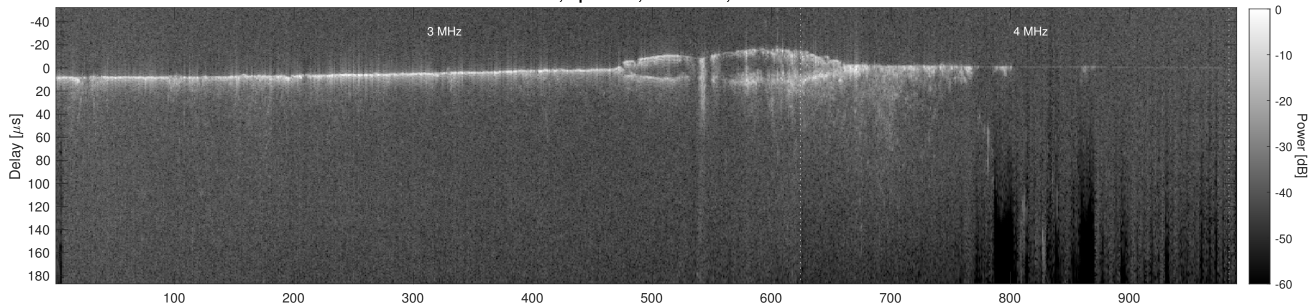
Orbit 9803, Cluttergram
