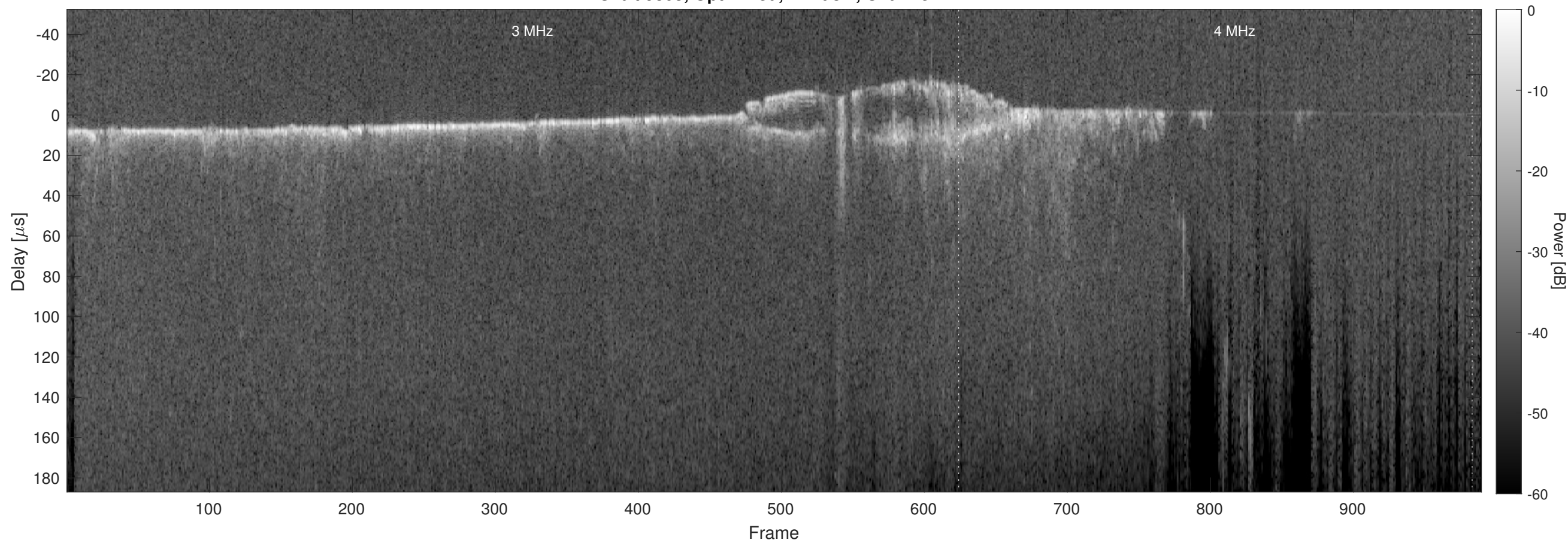
Orbit 9803, Optimized, Window, Channel 2
