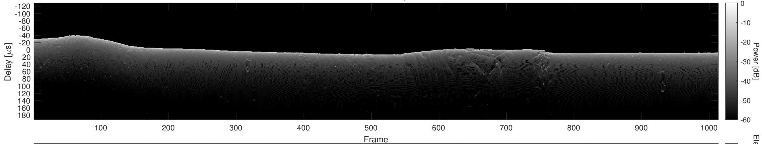
Orbit 9804, Cluttergram
