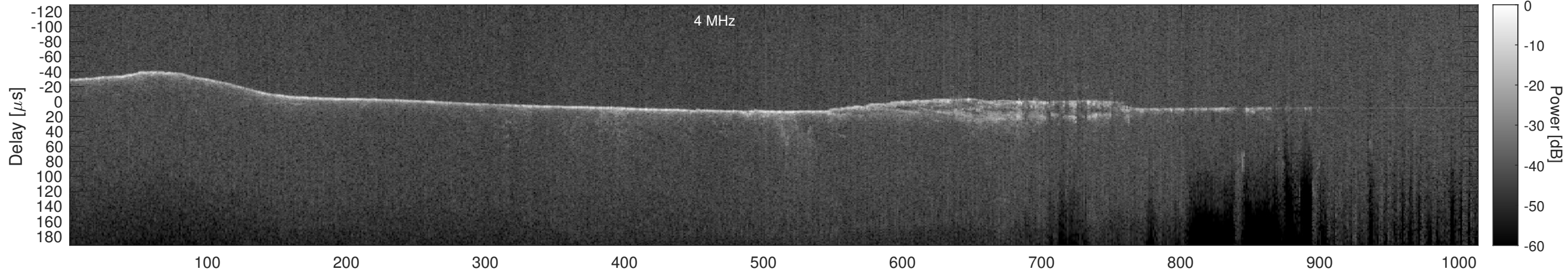
Orbit 9804, Cluttergram
