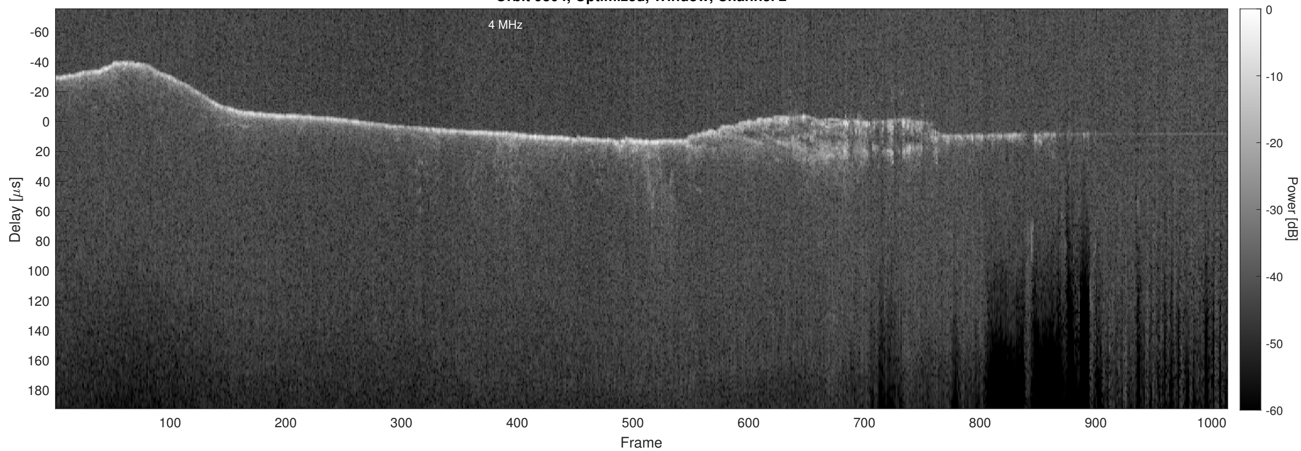
Orbit 9804, Optimized, Window, Channel 2
