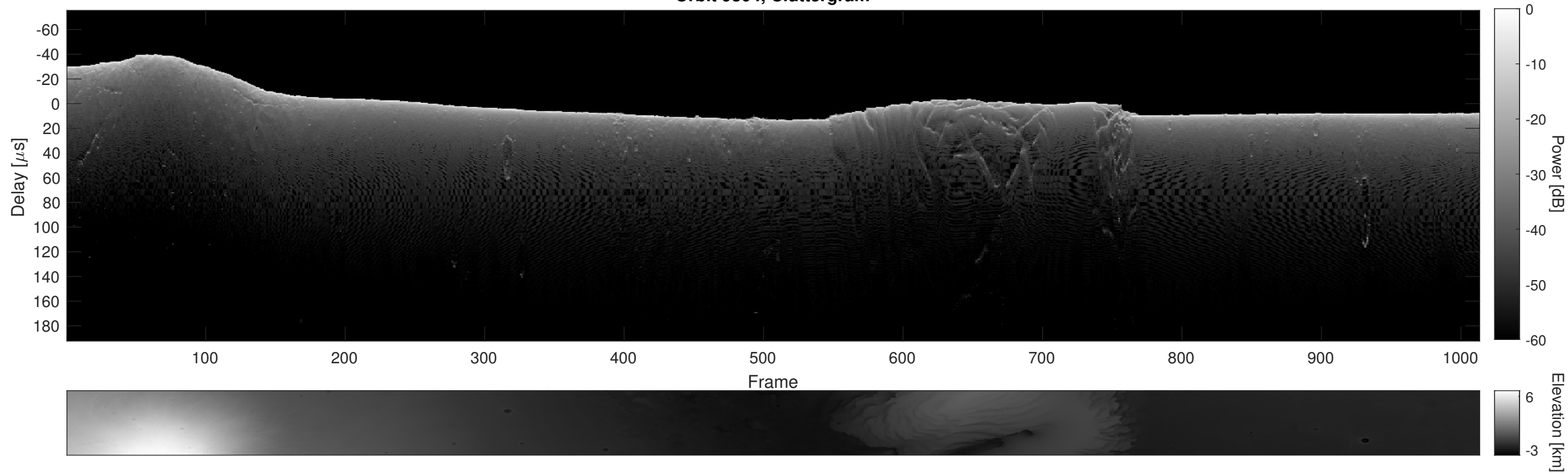
Orbit 9804, Cluttergram
