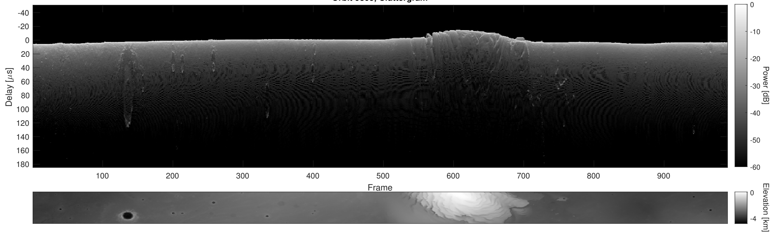
Orbit 9805, Cluttergram
