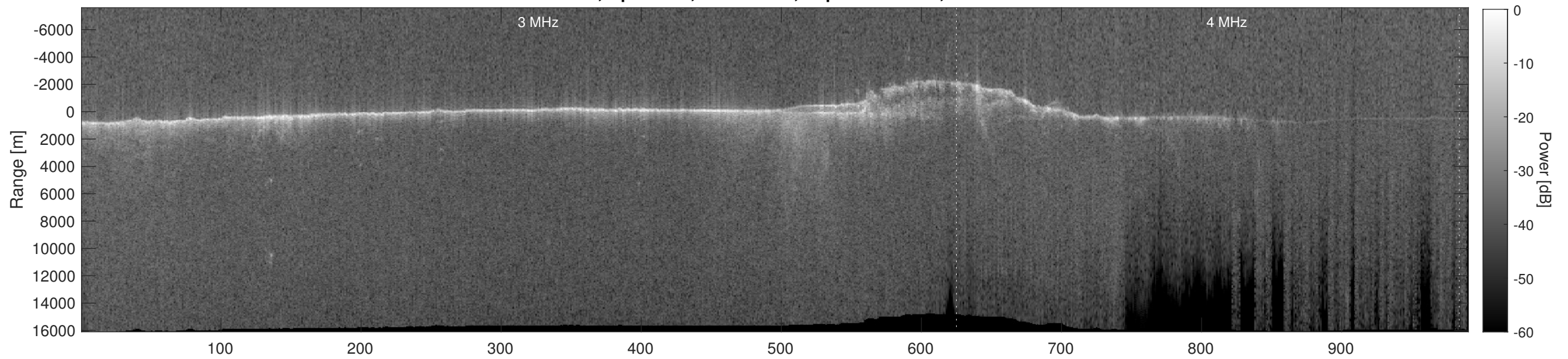
Orbit 9805, Depth-Corrected Cluttergram
