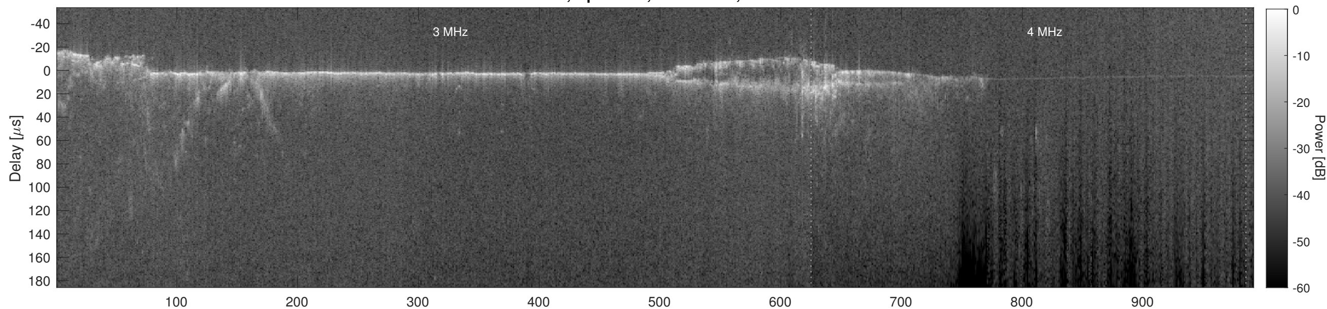
Orbit 9806, Cluttergram
