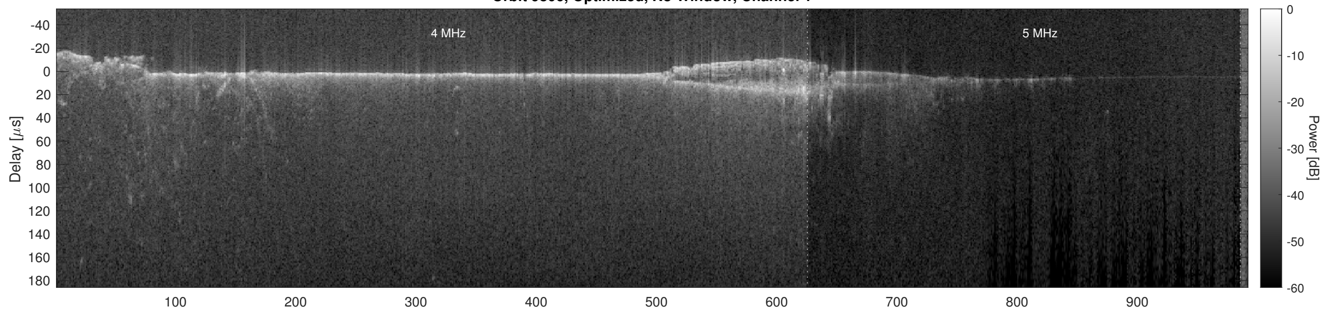
Orbit 9806, Optimized, No Window, Channel 2
