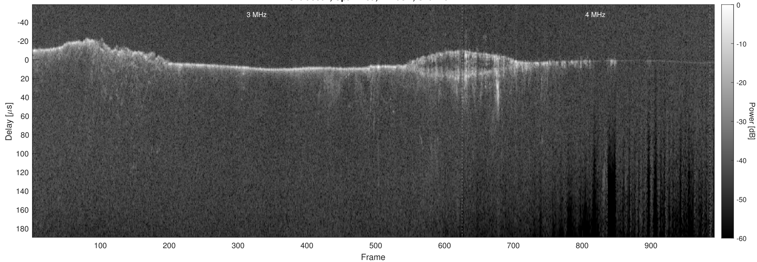
Orbit 9807, Optimized, Window, Channel 2
