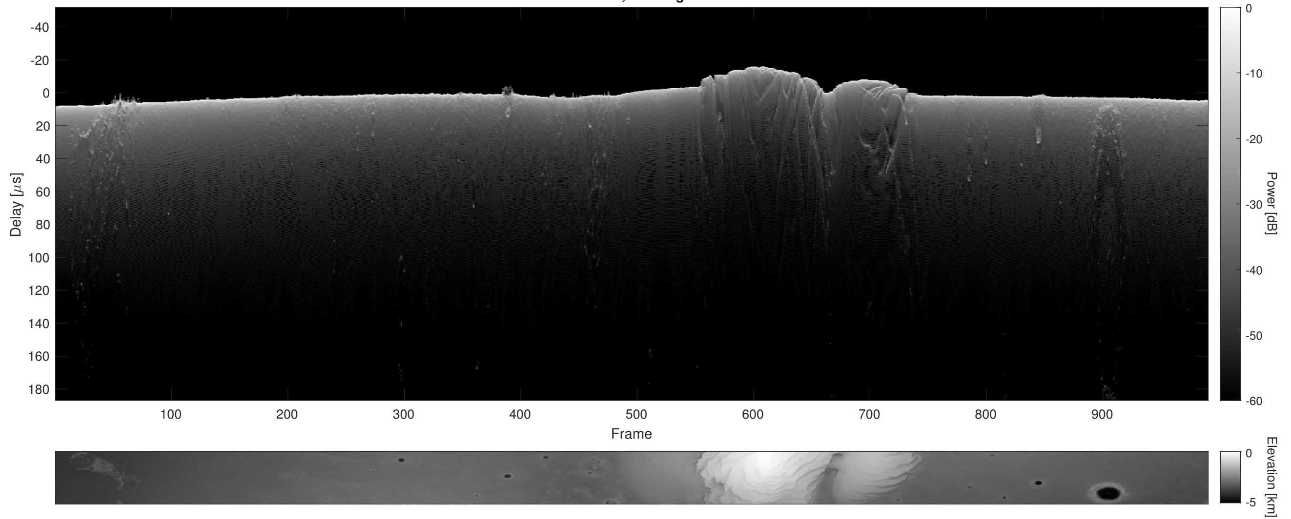
Orbit 9808, Cluttergram
