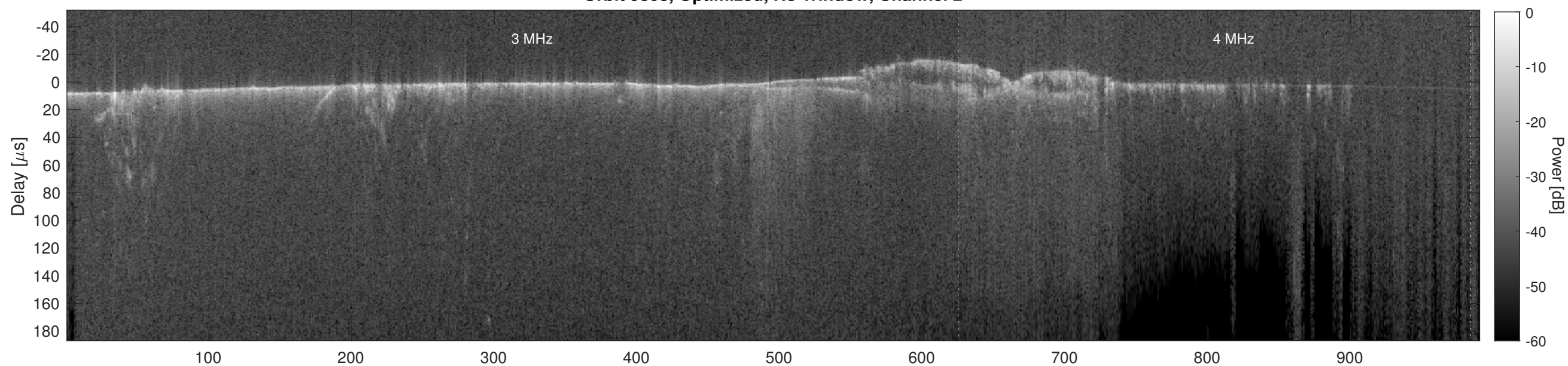
Orbit 9808, Cluttergram
