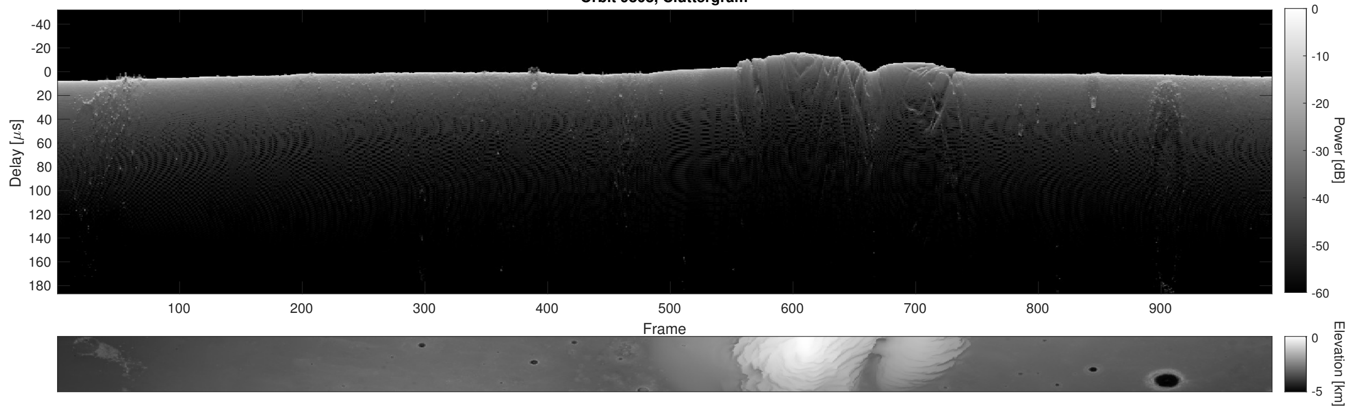
Orbit 9808, Cluttergram
