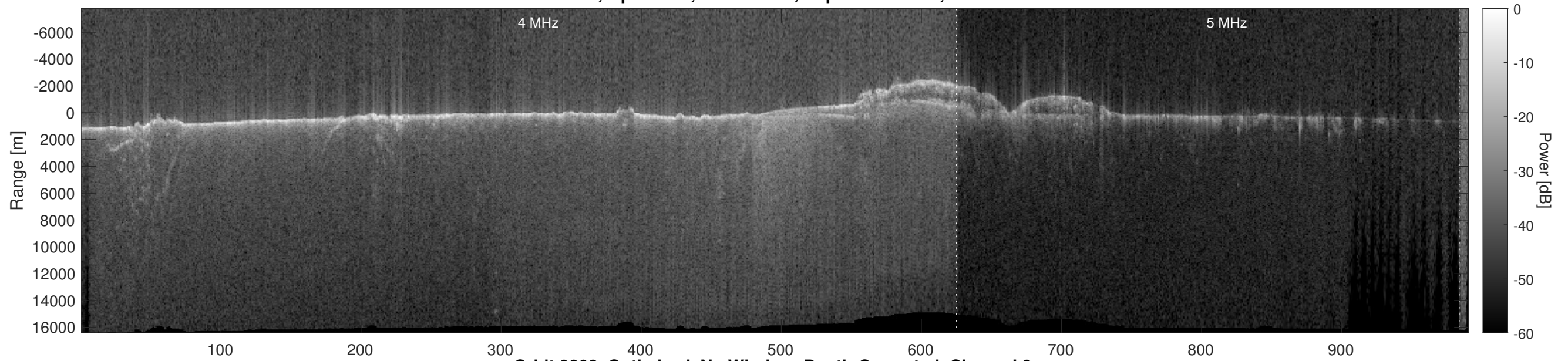
Orbit 9808, Optimized, No Window, Depth-Corrected, Channel 2
