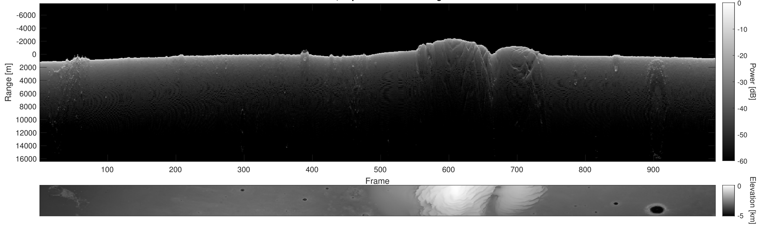
Orbit 9808, Depth-Corrected Cluttergram
